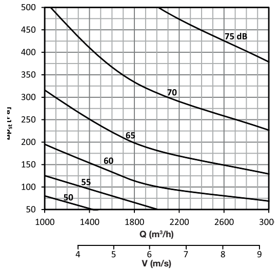
DAC-R 300 x 300
