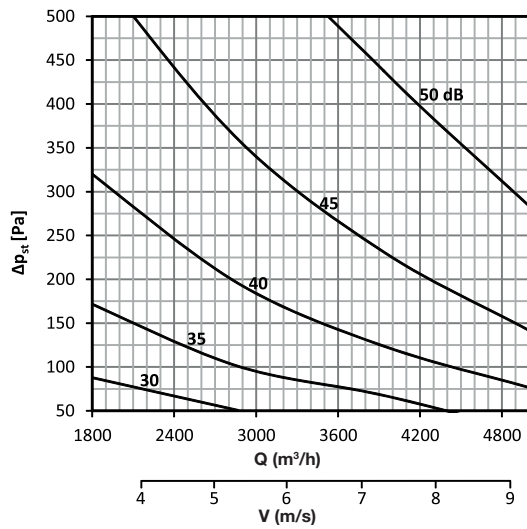
DAC-R 600 x 250
