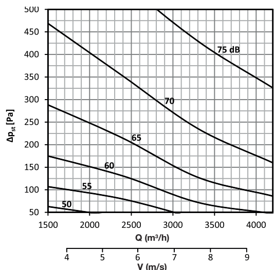
DAC-R 400 x 300
