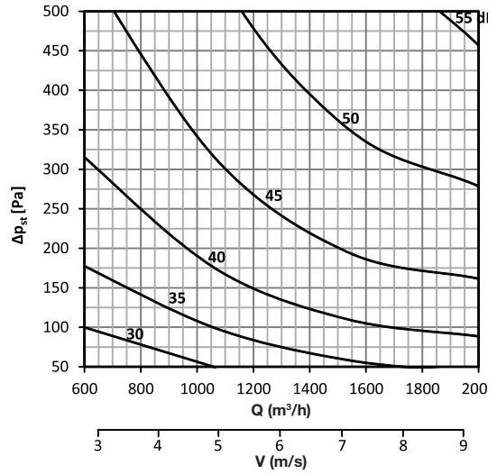
DAC-R 300 x 200
