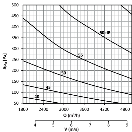
DAC-R 600 x 250
