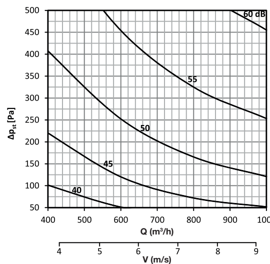
DAC-R 300 x 100
