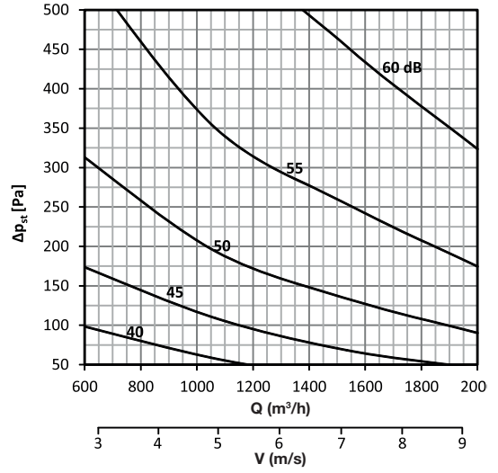
DAC-R 300 x 200
