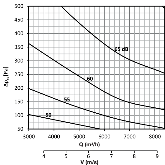
DAC-R 500 x 500
