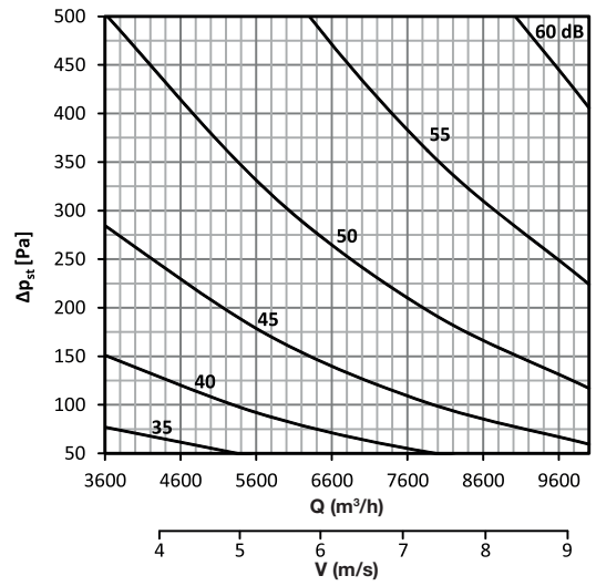
DAC-R 600 x 500
