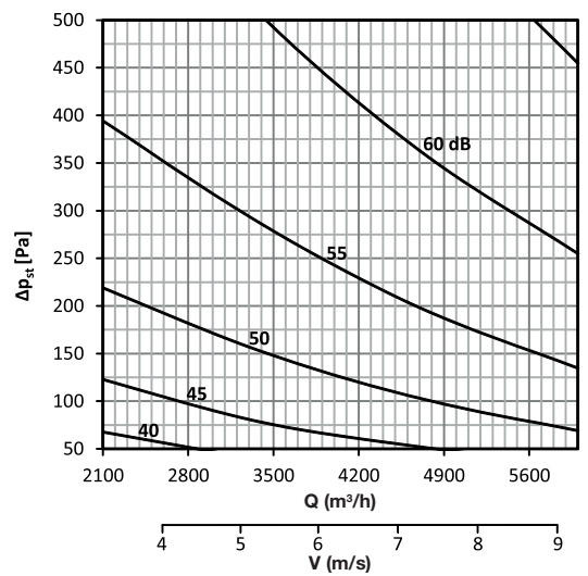
DAC-R 600 x 300
