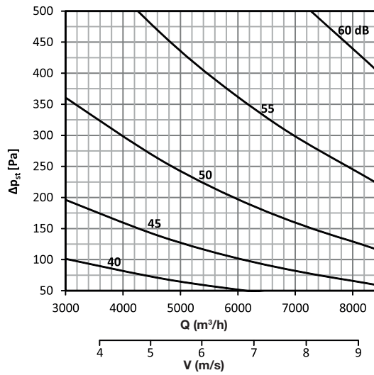
DAC-R 500 x 500
