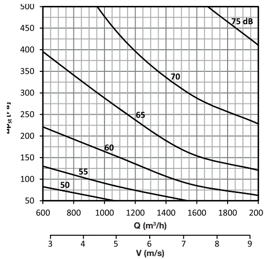
DAC-R 300 x 200
