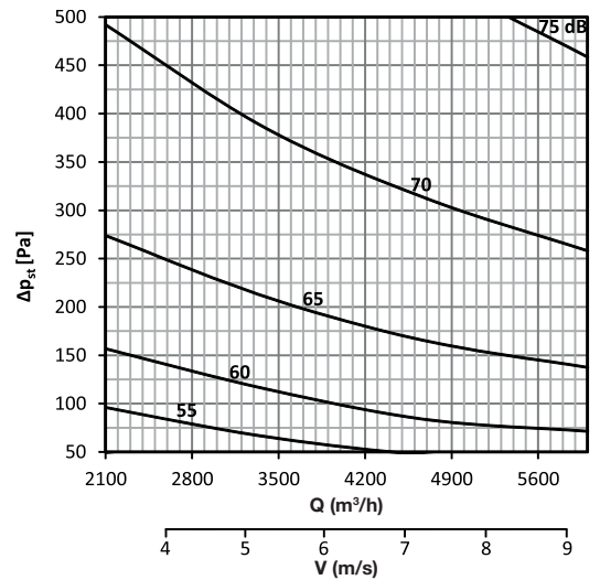
DAC-R 600 x 300
