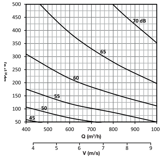
DAC-R 200 x 150
