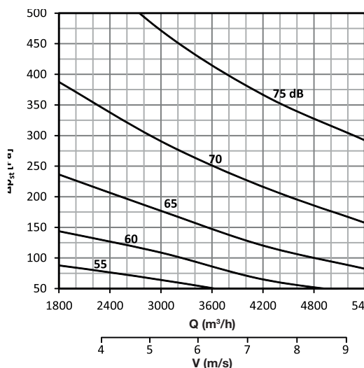
DAC-R 400 x 400
