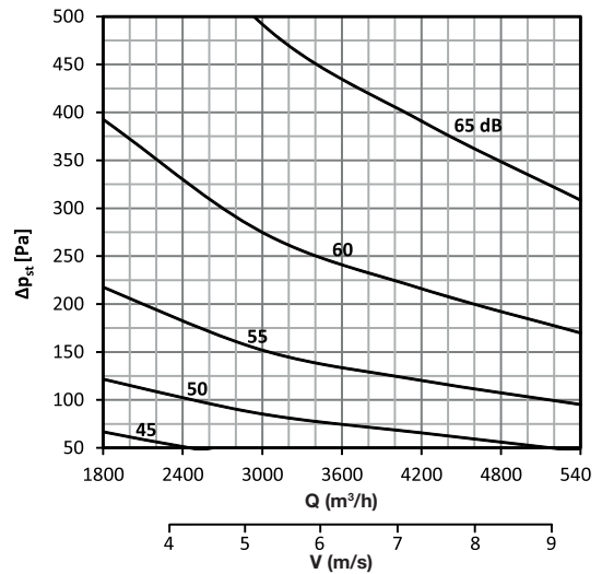
DAC-R 400 x 400
