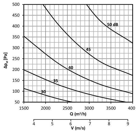
DAC-R 600 x 200
