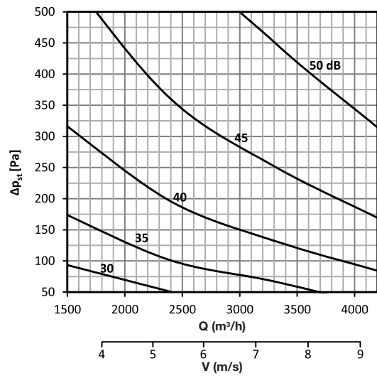
DAC-R 500 x 250
