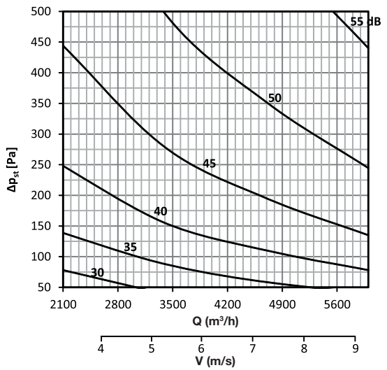
DAC-R 600 x 300
