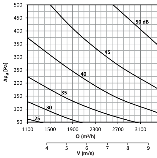
DAC-R 500 x 200
