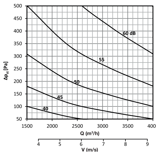
DAC-R 600 x 200
