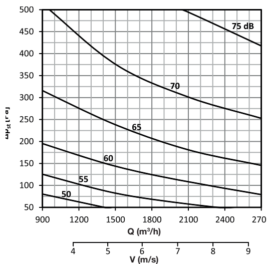
DAC-R 400 x 200
