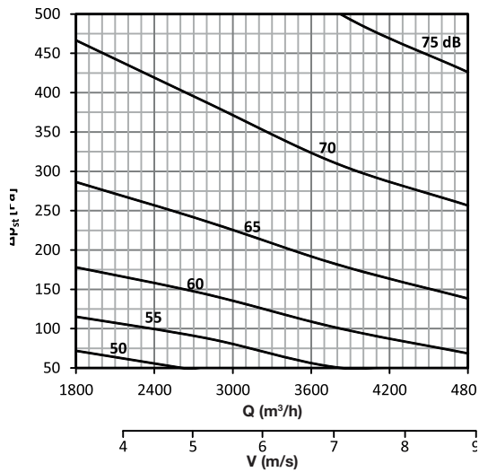
DAC-R 500 x 300
