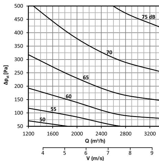
DAC-R 400 x 250
